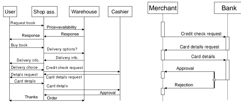
Fig. 1. Example Interaction Diagram (left) and Protocol (right)
